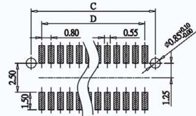
Recommended PCB Layout (PCB TOLERANCE \pm 0.05 )
