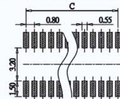
Recommended PCB Layout (PCB TOLERANCE ±0.05)
