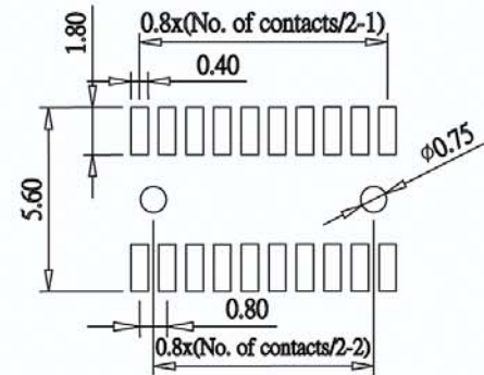
Recommended PCB Layout (PCB TOLERANCE \pm 0.05 )
